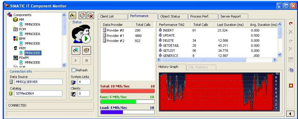
Component Monitor – Performance
