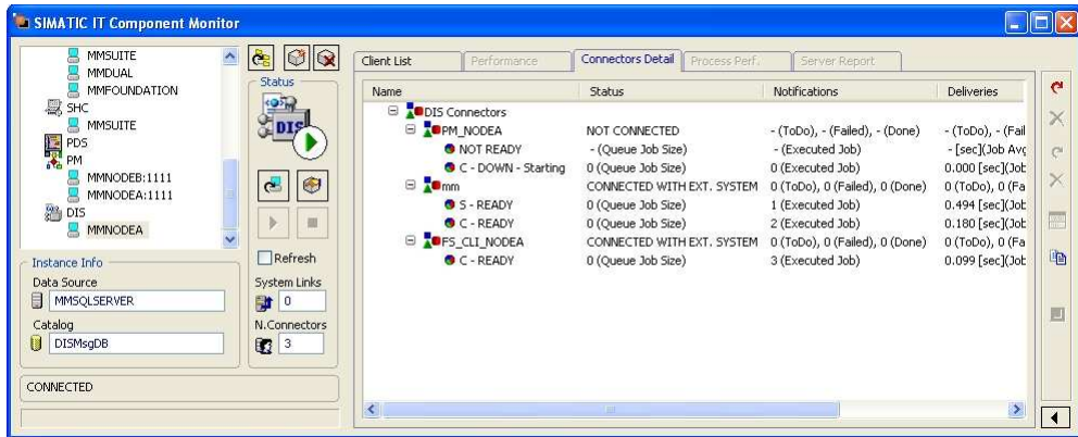
Component Monitor – Obj Info
